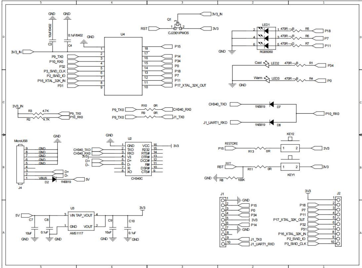
Figure 8 Schematic diagram of the development board
