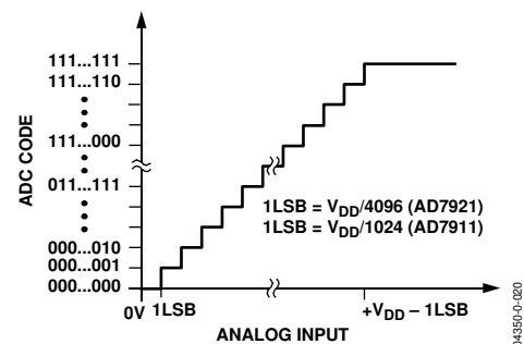
Figure 21. AD7911/AD7921 Transfer Characteristic
