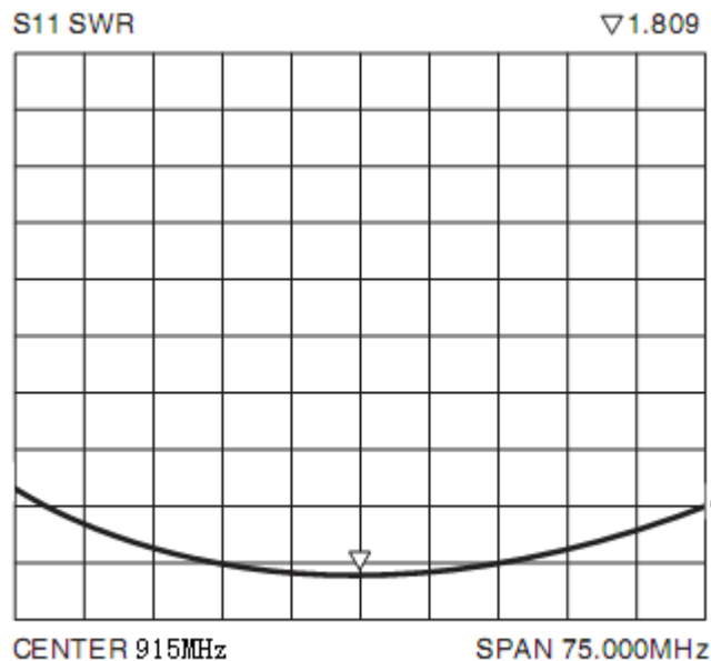
Typical VSWR
