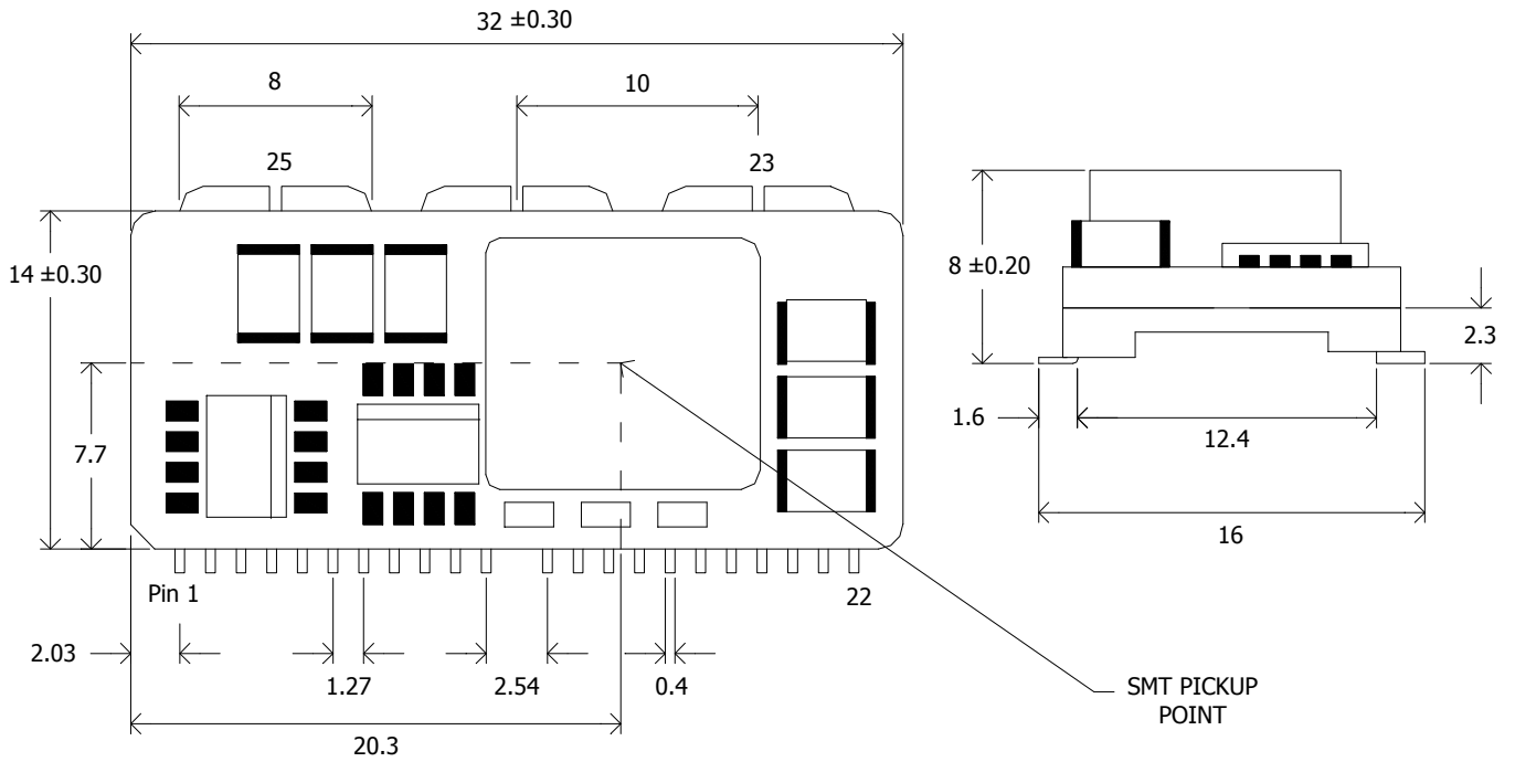
Figure 57. Mechanical Drawing
