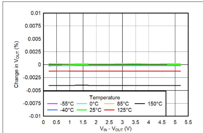
Figure 6-23. V_{IN} Line Regulation
