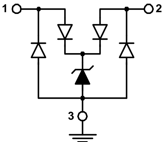
Circuit Diagram
