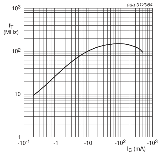
Fig 45. PDTB143XU: Transition frequency as a function of collector current; typical values of built-in transistor
