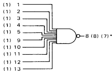
MC1804/MC1904 MC1805/MC1905 10-Input NAND Gate
