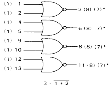
MC1810/MC1910 MC1811/MC1911 Quad 2-Input NOR Gate
