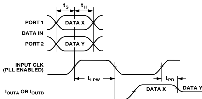
Figure 1. I/O Timing
