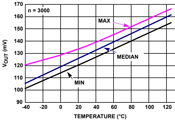
FIGURE 33. ISL28271 V_{OUT} LOW vs TEMPERATURE, R_L = 1k , V_+ = V_- = \pm 2.5V
