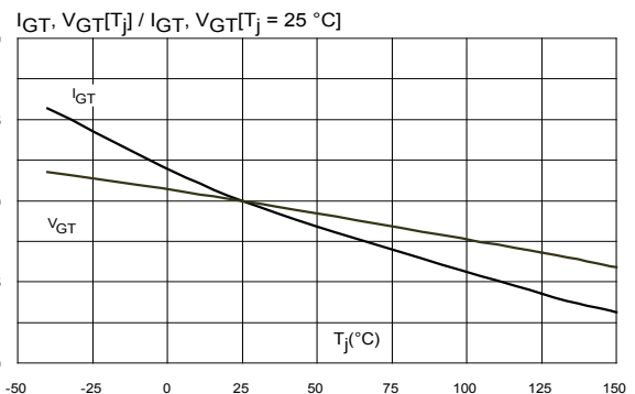
Figure 6. Relative variation of gate trigger current and gate voltage versus junction temperature
