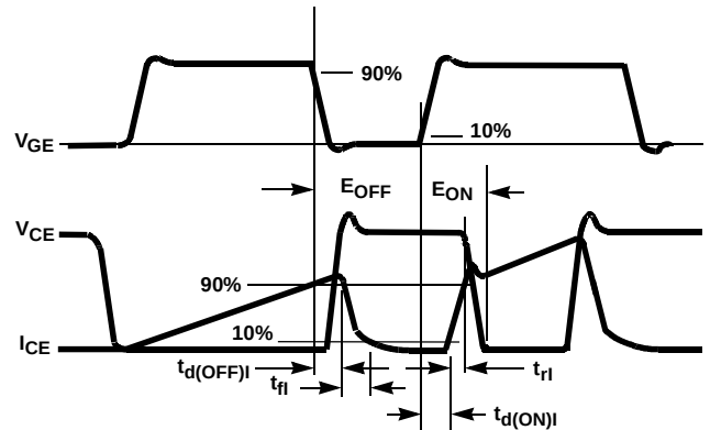
FIGURE 17. SWITCHING TEST WAVEFORMS
