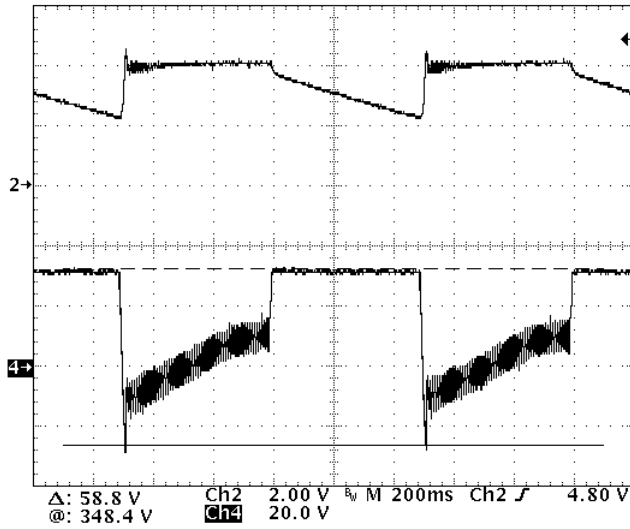
Figure 14. Load Transient (Load step: 0% to 100%. Ch. 2 = VCOMP @ 2 V/div., Ch. 4 = V OUT @ 10 V/div. offset by 375 VDC)
