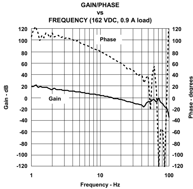
Figure 16. Bode Plot (162 VDC input, full load. Crossover frequency = 13 Hz, phase margin = 68°)
