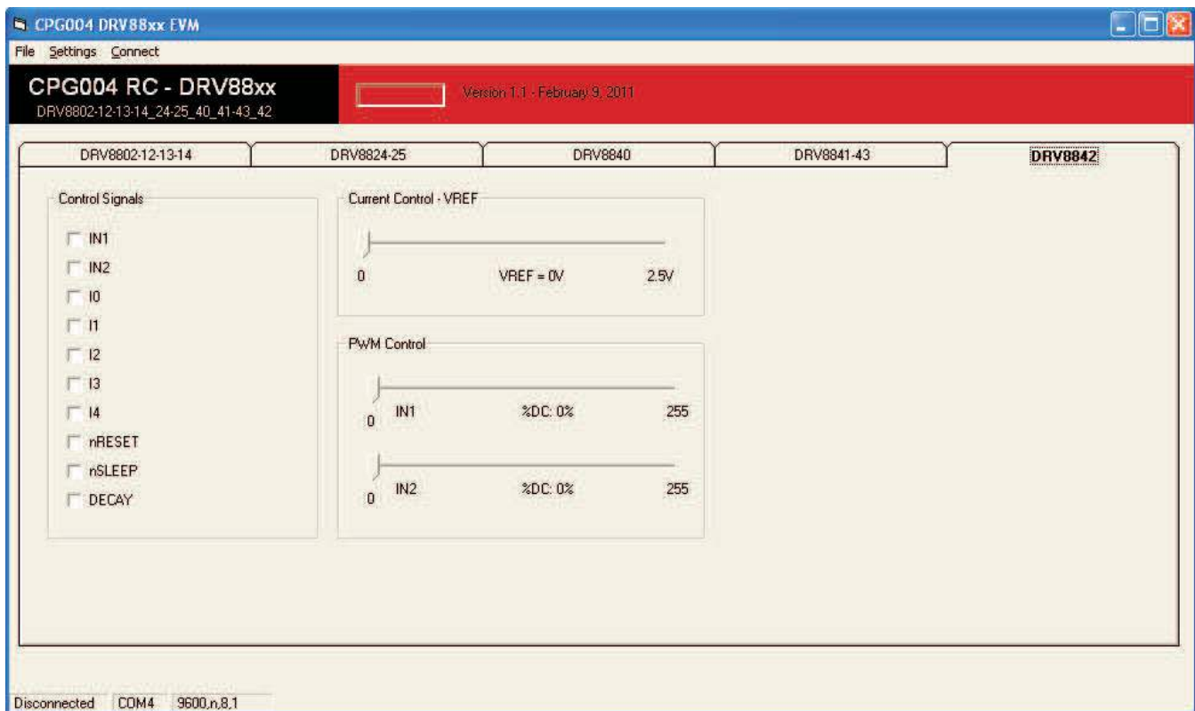
Figure 4. DRV8842 Tab
