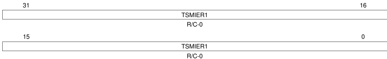
Figure 23-88. Transfer to System Memory Interrupt Enable Reset 1 (TSMIER1) [offset_TU = 104h]
