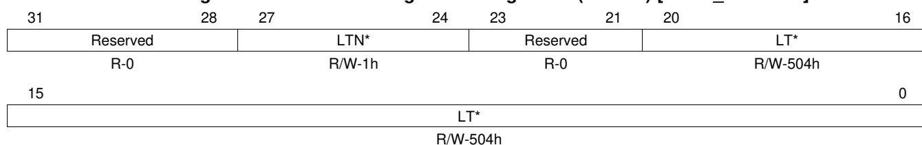
Figure 23-122. SUC Configuration Register 2 (SUCC2) [offset_CC = 84h]
