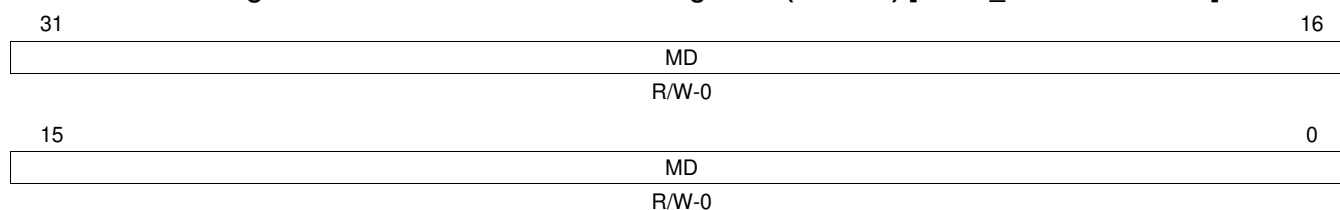
Figure 23-173. Write Data Section Registers (WRDSn) [offset_CC = 400h-4FCh]
