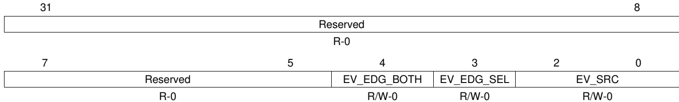
Figure 19-28. ADC Event Group Trigger Source Select Register (ADEVSR) [offset = 1Ch]
