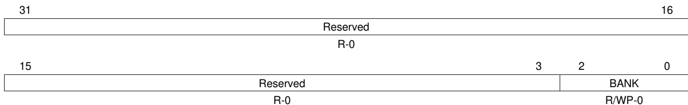
Figure 5-26. Flash Module Access Control Register (FMAC) [offset = 50h]
