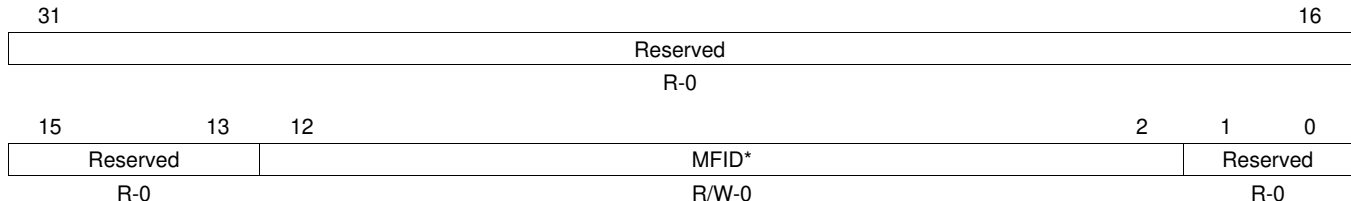
Figure 23-153. FIFO Rejection Filter Mask Register (FRFM) [offset_CC = 308h]
