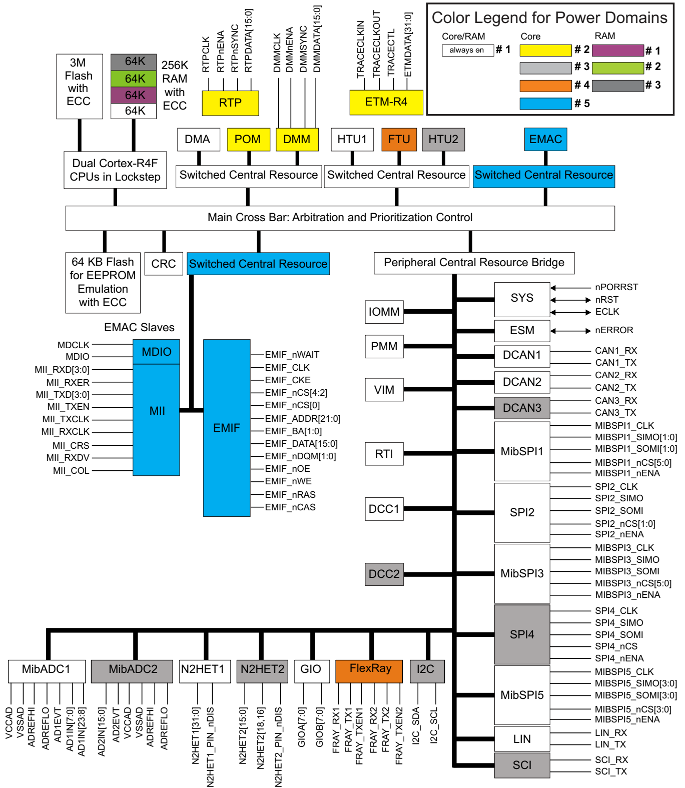
Figure 1-1. Block Diagram
