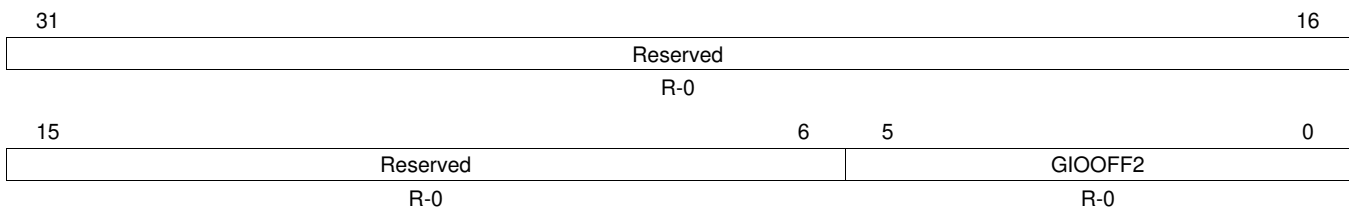
Figure 22-14. GIO Offset 2 Register (GIOOFF2) [offset = 28h]
