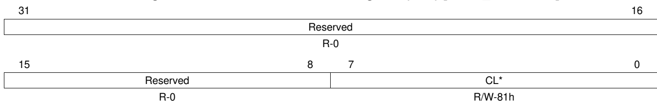
Figure 23-154. FIFO Critical Level Register (FCL) [offset_CC = 30Ch]
