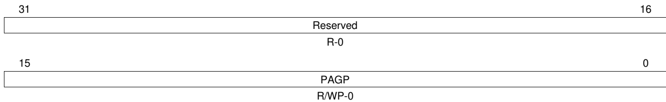
Figure 5-25. Flash Pump Access Control Register 2 (FPAC2) [offset = 4Ch]
