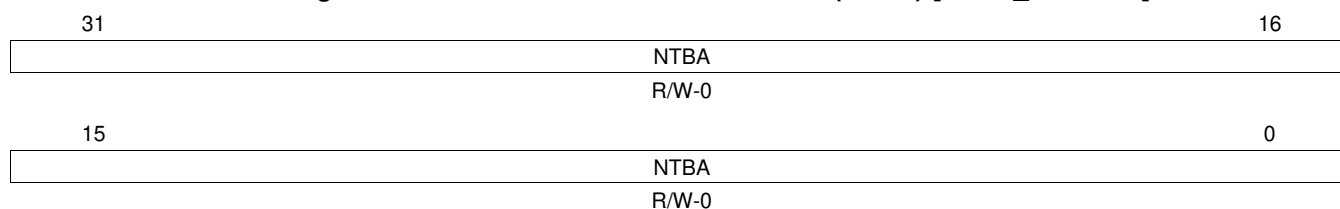
Figure 23-38. Next Transfer Base Address (NTBA) [offset_TU = 28h]
