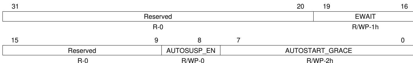
Figure 5-40. EEPROM Emulation Configuration Register (EEPROM_CONFIG) [offset = 2B8h]
