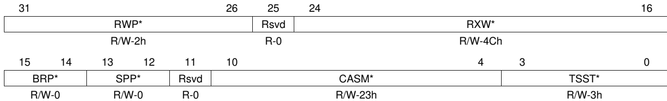
Figure 23-125. PRT Configuration Register 1 (PRTC1) [offset_CC = 90h]
