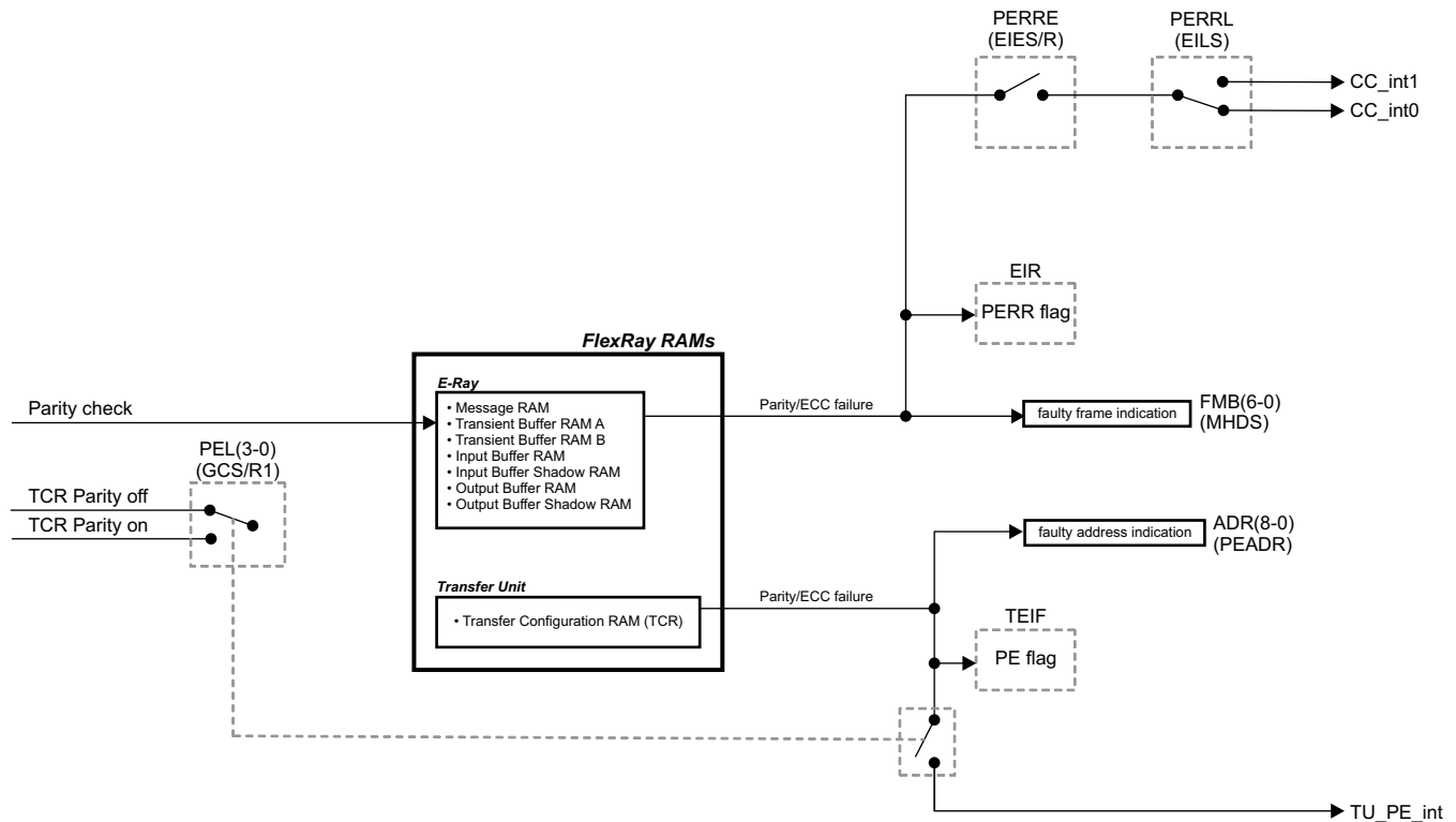
Figure 23-26. Parity Structure
