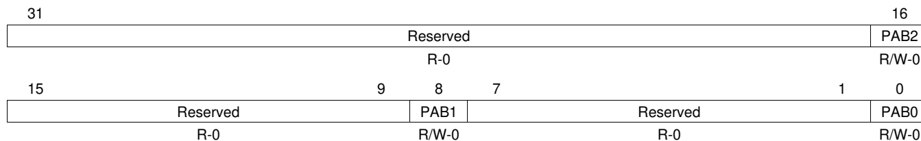
Figure 23-104. Parity Information in TCR Parity Test Mode [offset_TU_RAM = 200h-3FFh]
