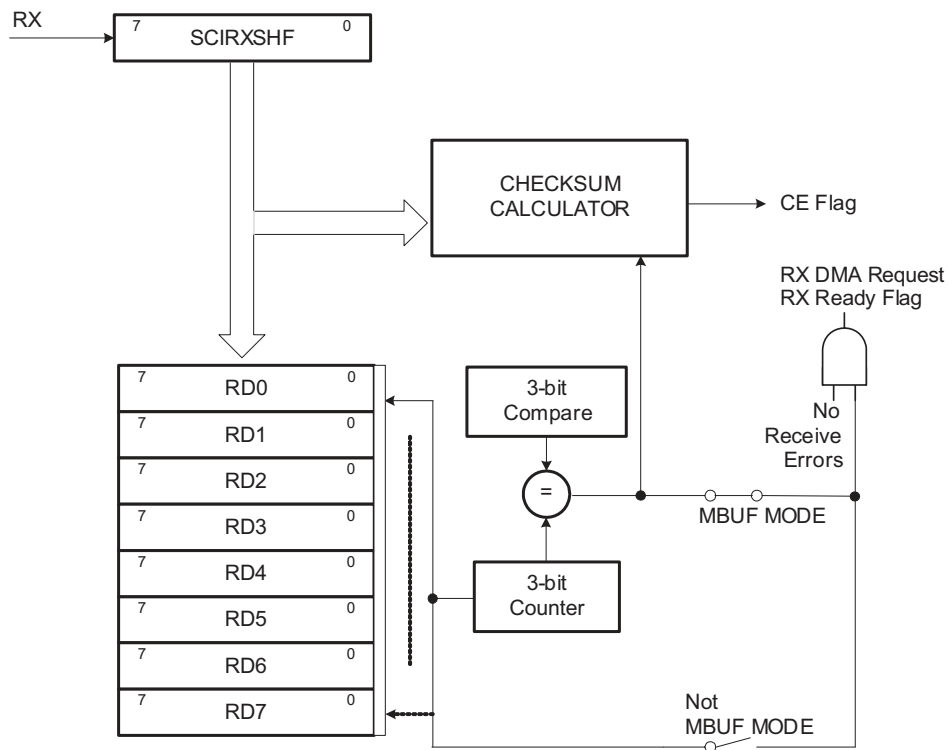
Figure 26-8. Receive Buffers
