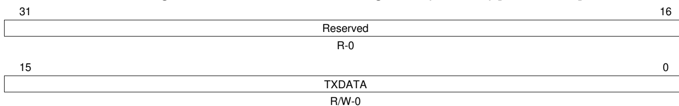
Figure 25-40. SPI Transmit Data Register 0 (SPIDAT0) [offset = 38h]
