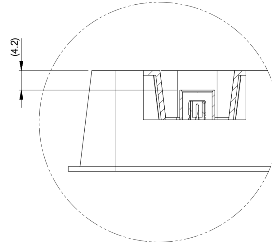
DETAIL F SCALE 2:1
