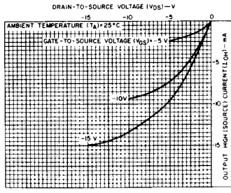
Fig. 9 - Minimum output high (source) current characteristics.
