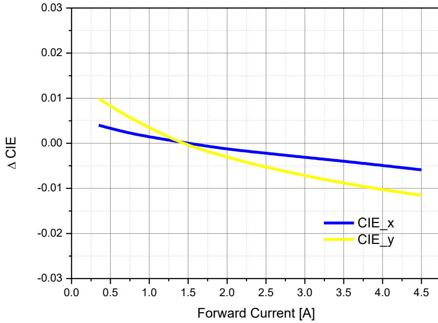
Forward Current vs \Delta CIE Tj=25°C (White)
