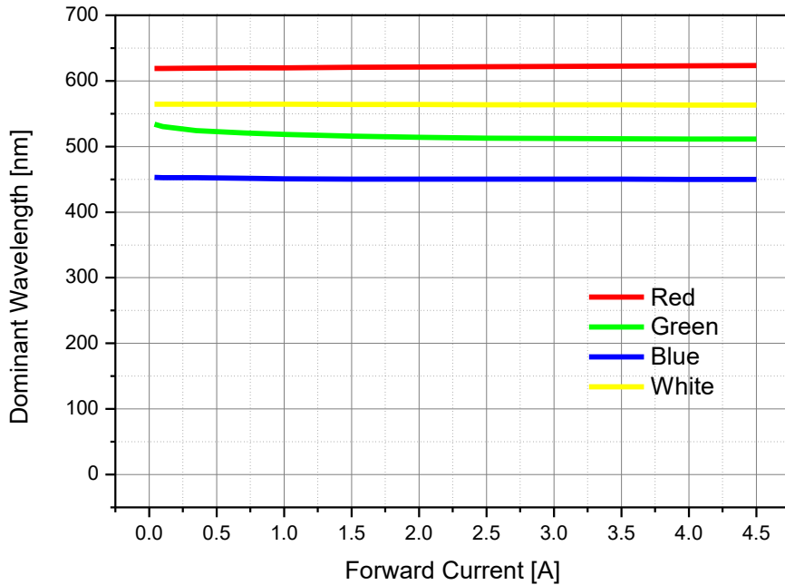
Forward Current vs Dominant Wavelength, T j =25°C
