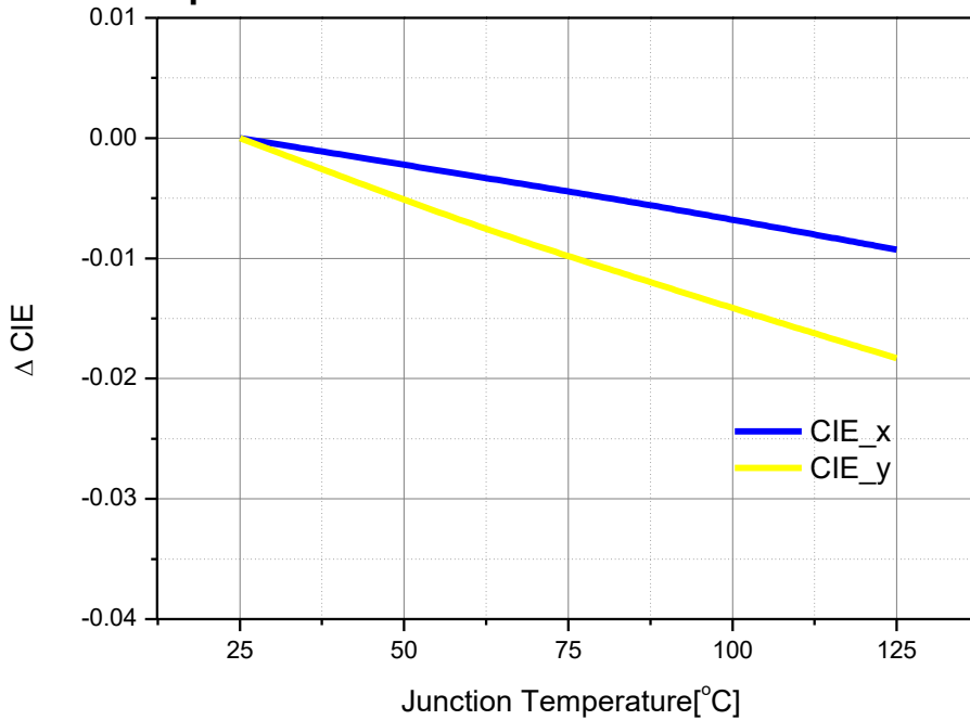
Junction Temperature vs. White ΔCIE at IF=1400mA
