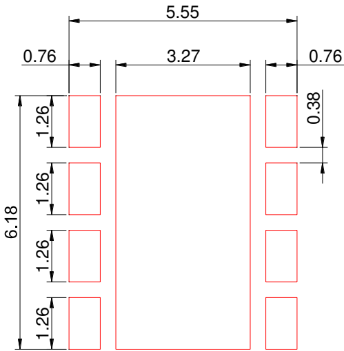
Recommended Solder Pad
