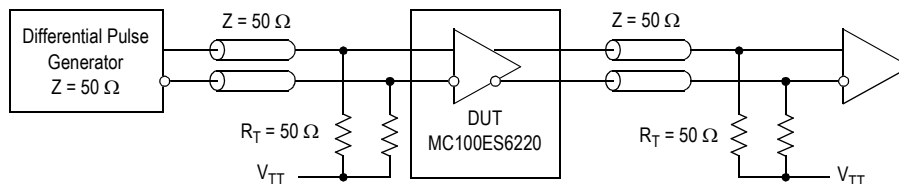
Figure 3. MC100ES6220 AC Test Reference
