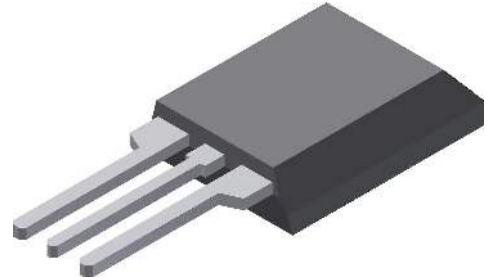
Backside: isolated
