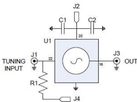
VOG SCHEMATIC
