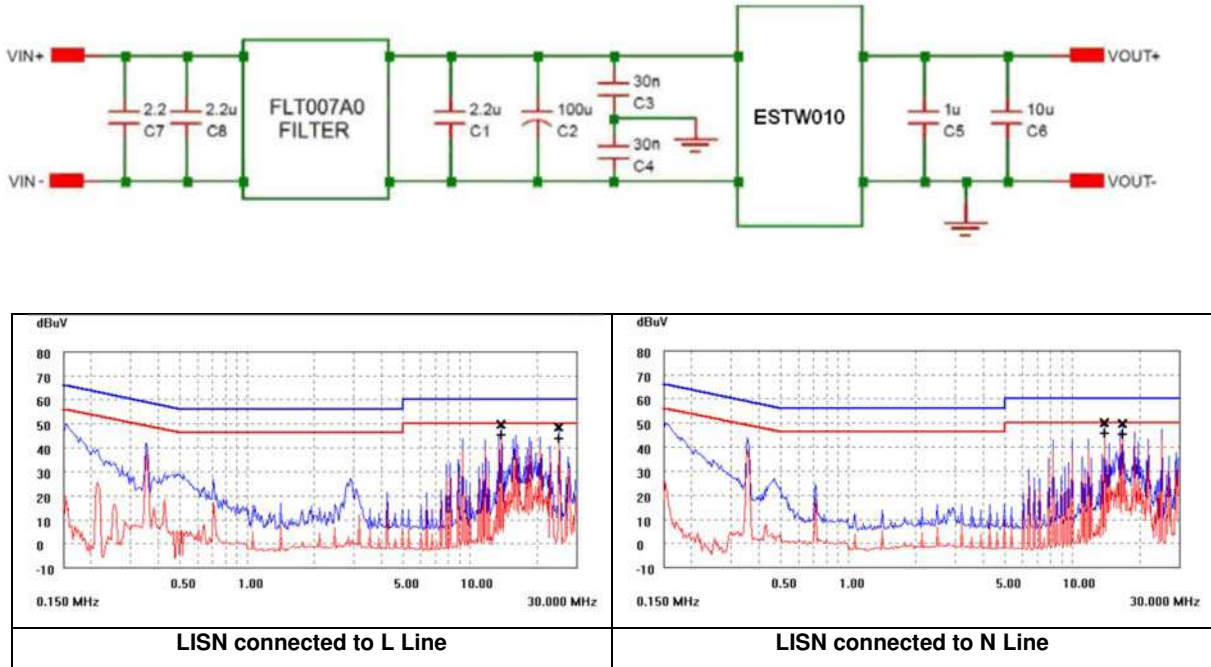
Figure 25. EMC Considerations
