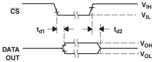
Figure 37. DATA OUT to Hi-Z Voltage Waveforms
