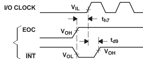
Figure 44. I/O CLOCK and EOC Voltage Waveforms
