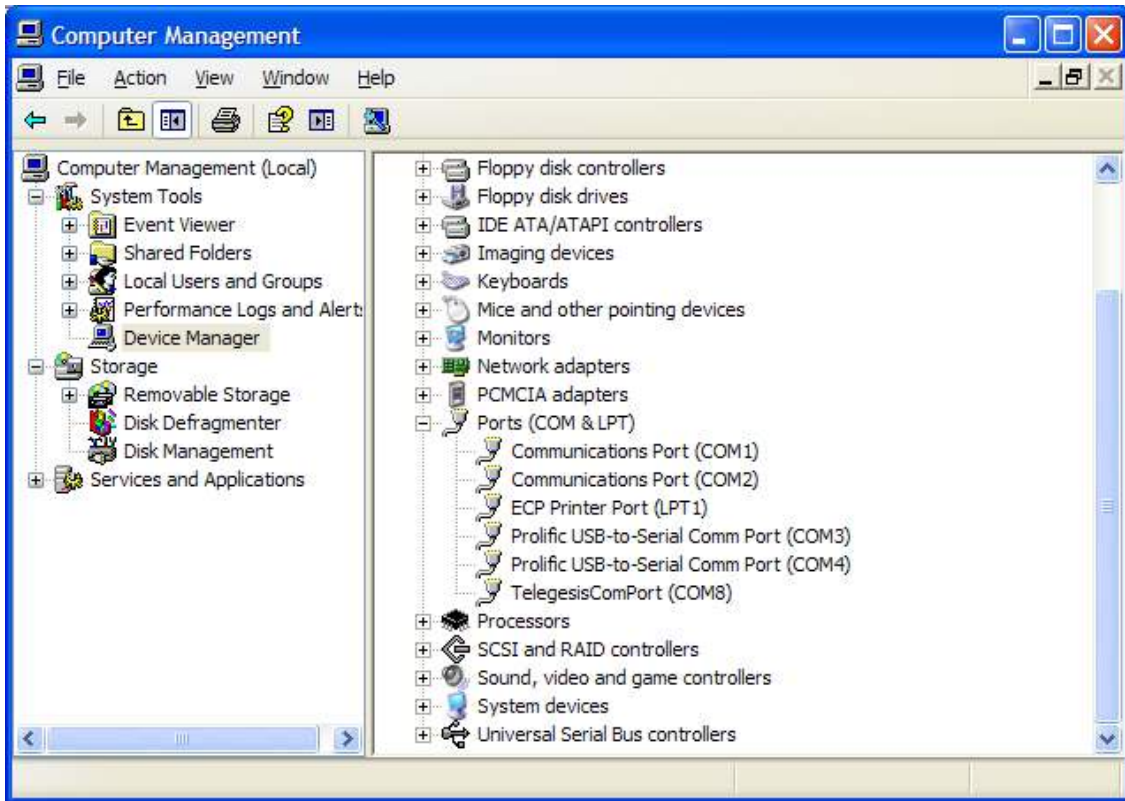
Figure 4. Device Manager
