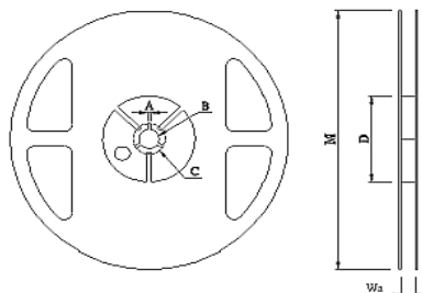
Reel Dimensions (mm)
