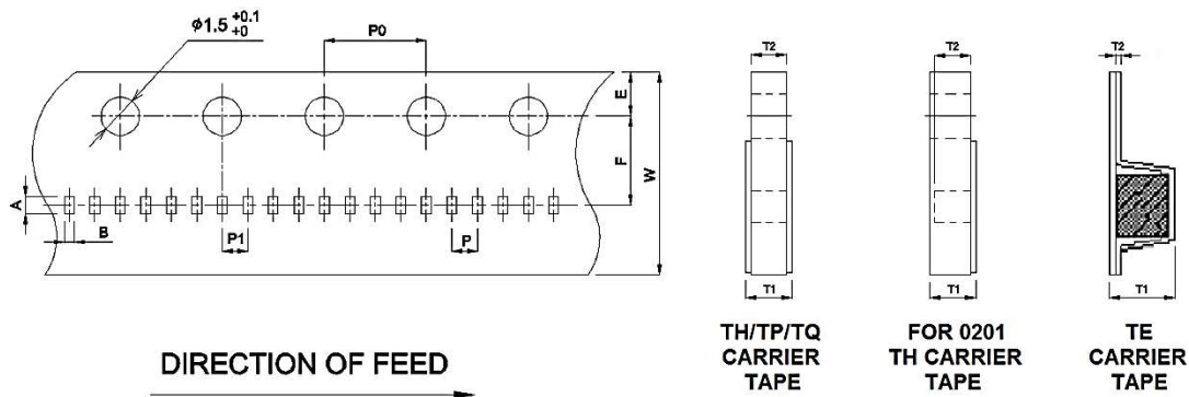
Tape Dimensions (mm)
