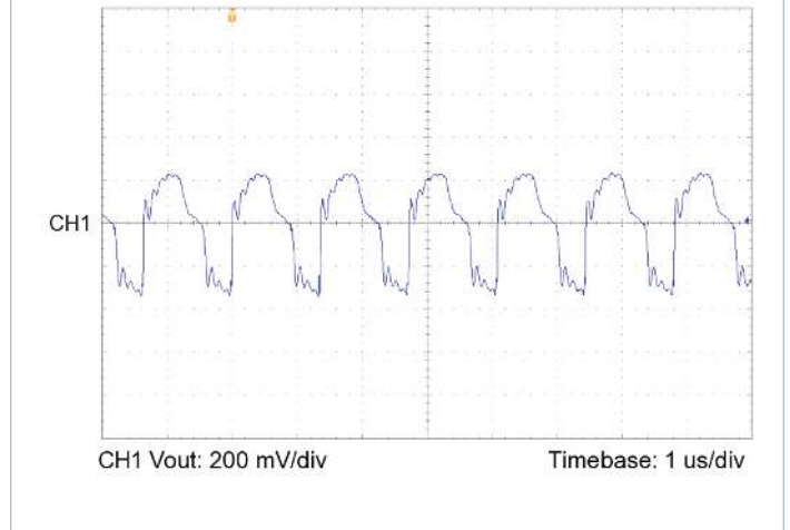
Figure 16 — Output voltage ripple, V_{IN} = 275\text{ V} , V_{OUT} = 15.0\text{ V} , C_{OUT\_EXT} = 1000\ \mu\text{F} , R_{LOAD} = 0.600\ \Omega
