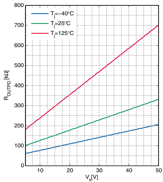
Internal output pull down resistor R_{OUTPDP} versus supply voltage V_S
