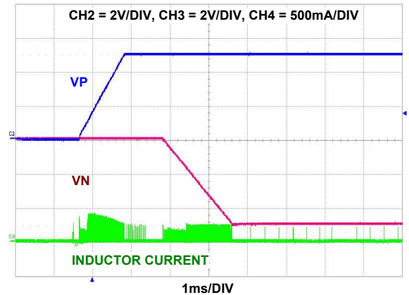
FIGURE 39. VP AND VN ( \pm 5\text{V} ) SOFT-START AT 5V INPUT VOLTAGE, VP/VN SEQUENCED (Reg 0x04 <b 4 > = 0)
