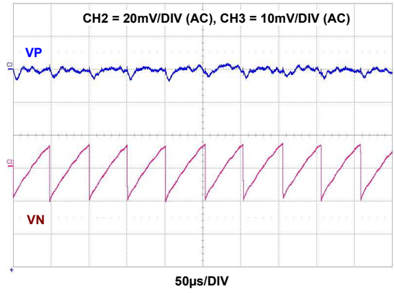
FIGURE 19. VP/VN (±5V) OUTPUT VOLTAGE RIPPLE, 2mA LOAD
