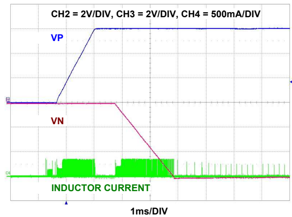
FIGURE 55. VP AND VN ( \pm 6\text{V} ) SOFT-START AT 5V INPUT VOLTAGE, VP/VN SEQUENCED (Reg 0x04 <b 4 > = 0)
