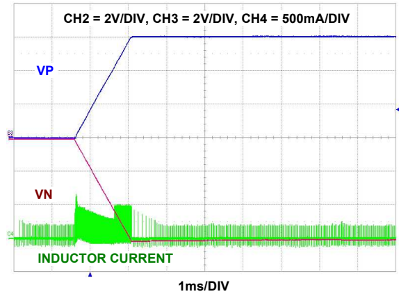
FIGURE 57. VP AND VN ( \pm 6\text{V} ) SOFT-START AT 2.5V INPUT VOLTAGE, VP/VN START TOGETHER (Reg 0x04 <b 4 > = 1)
