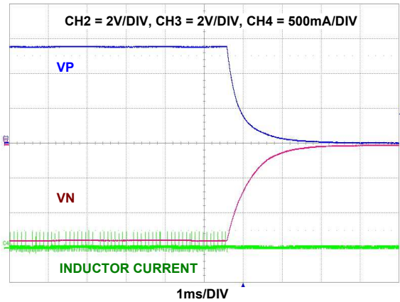
FIGURE 52. VP AND VN ( \pm 5.5\text{V} ) SHUTDOWN, VP/VN SHUTDOWN TOGETHER (Reg 0x05 <b 4 > = 1)
