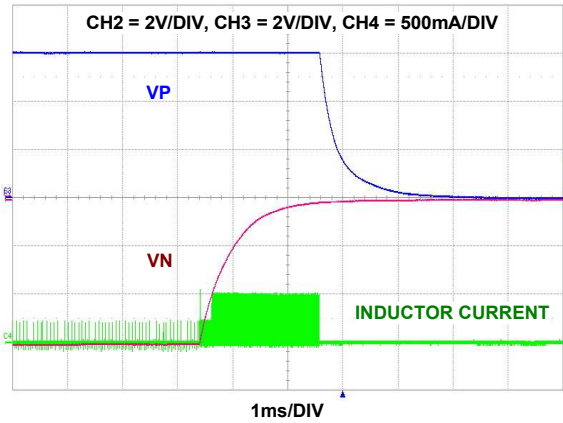
FIGURE 56. VP AND VN ( \pm 6\text{V} ) SHUTDOWN, VP/VN SEQUENCED (Reg 0x05 <b 4 > = 0)
