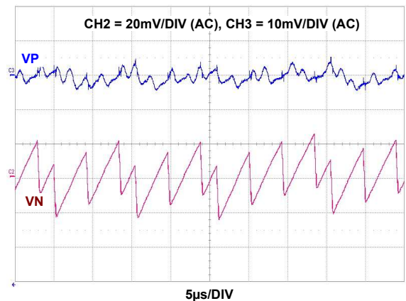
FIGURE 21. VP/VN (±5V) OUTPUT VOLTAGE RIPPLE, 30mA LOAD
