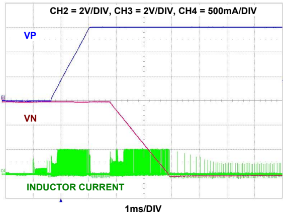
FIGURE 54. VP AND VN ( \pm 6\text{V} ) SOFT-START AT 3.7V INPUT VOLTAGE, VP/VN SEQUENCED (Reg 0x04 <b 4 > = 0)
