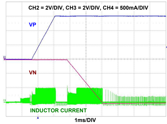
FIGURE 53. VP AND VN ( \pm 6\text{V} ) SOFT-START AT 2.5V INPUT VOLTAGE, VP/VN SEQUENCED (Reg 0x04 <b 4 > = 0)
