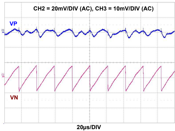
FIGURE 20. VP/VN (±5V) OUTPUT VOLTAGE RIPPLE, 5mA LOAD
