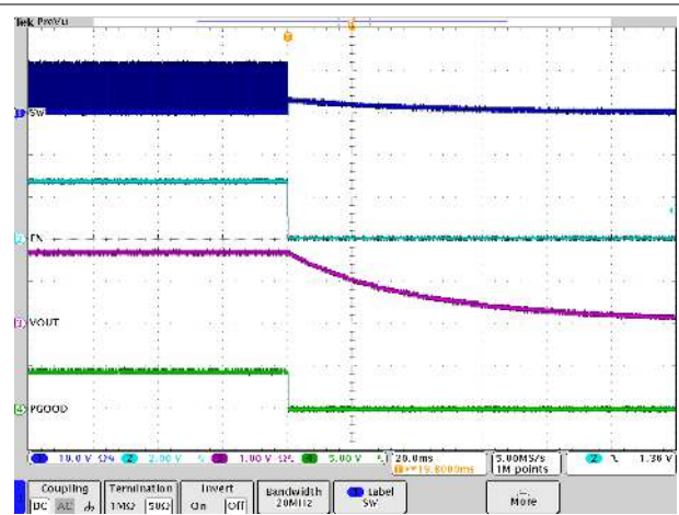
Figure 2-14. ENABLE Shutdown Waveform
