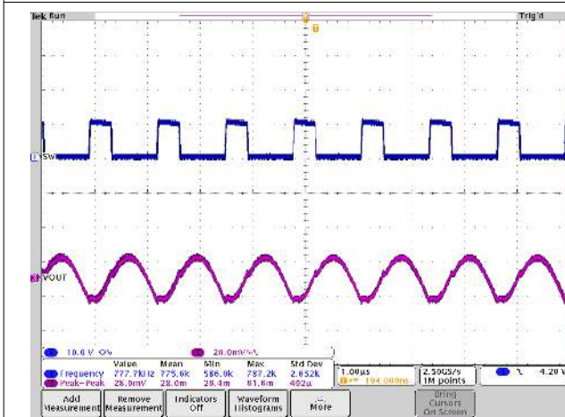
Figure 2-15. Output Voltage Ripple, 800-kHz FCCM, 35-A Load
