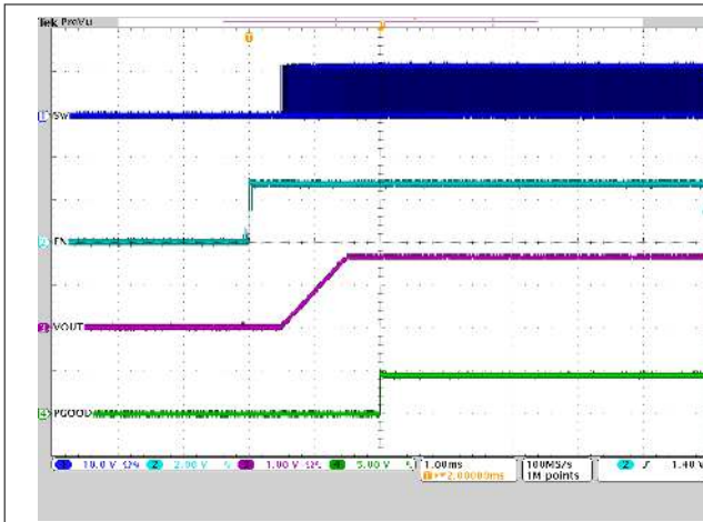
Figure 2-13. ENABLE Start-Up Waveform
