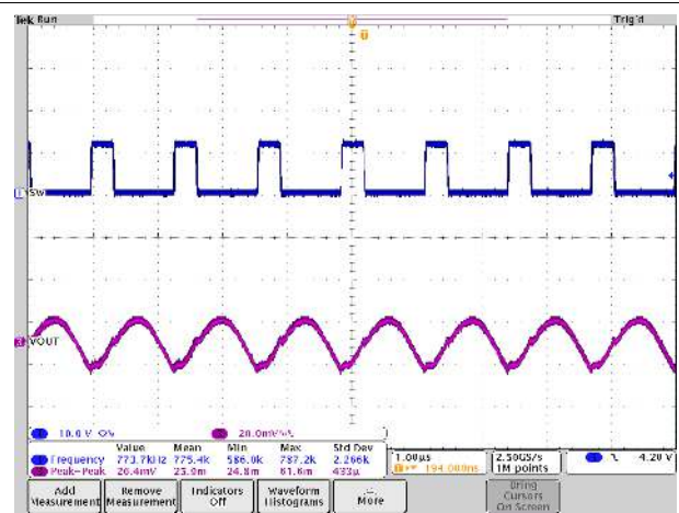
Figure 2-16. Output Voltage Ripple, 800-kHz FCCM, No Load
