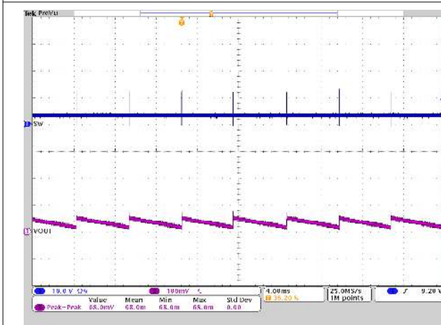
Figure 2-17. Output Voltage Ripple, DCM, No Load
