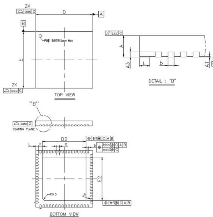
Figure 5.3. QFN64
