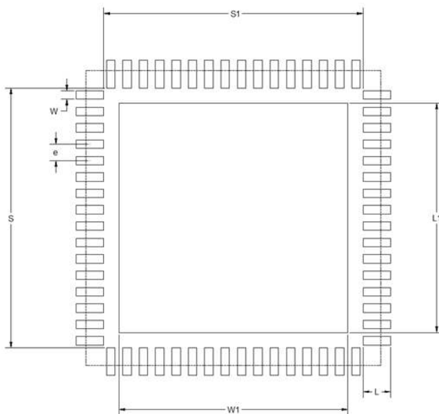
Figure 6.1. PCB Land Pattern
