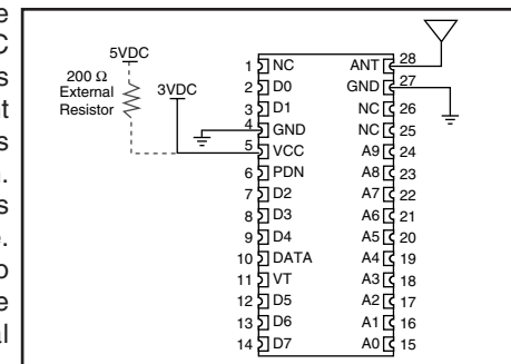
Figure 2: Test/Basic Application Circuit
