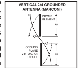
Figure 21: Dipole Antenna
