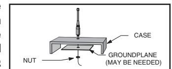
Figure 22: Remote Groundplane
