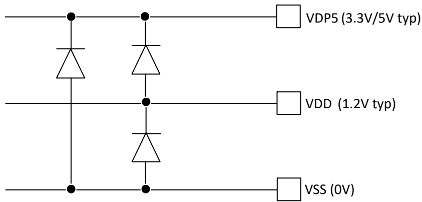
Figure 24. ESD Diodes between VDP5, VDD and VSS
