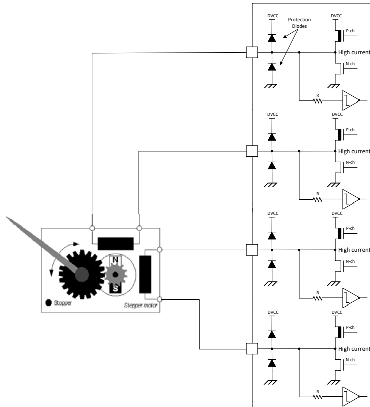
Figure 6. ESD Protection Structure for SMC Pins
