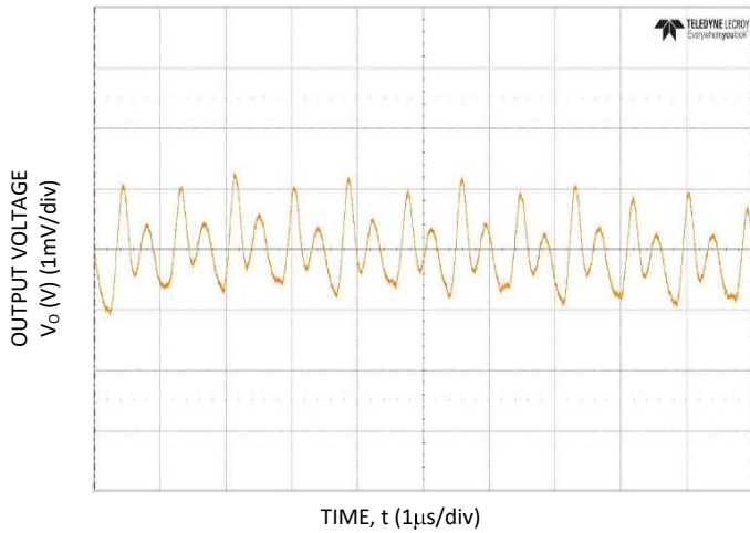
Figure 9. Typical output ripple (C o =4x0.047µF + 4x0.1µF + 15x22µF + 73x47µF + 6x470µF polymer, V IN = 12V, I o = I o,max ).
