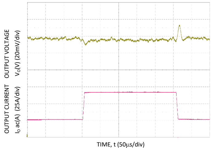
Figure 4. Trans. Resp. to 10A/µs Load Change from 25% to 75% at 12VIN, C_o=4 \times 0.047 \mu\text{F} + 4 \times 0.1 \mu\text{F} + 15 \times 22 \mu\text{F} + 73 \times 47 \mu\text{F} + 6 \times 470 \mu\text{F} polymer
