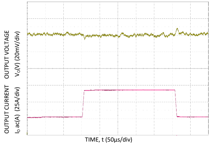
Figure 10. Trans. Resp. to 10A/µs Load Change from 25% to 75% at 12VIN, C o =4x0.047µF + 4x0.1µF + 15x22µF + 73x47µF + 6x470µF polymer
