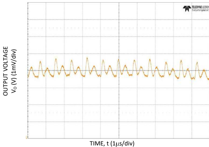
Figure 3. Typical output ripple ( C_o=4 \times 0.047 \mu\text{F} + 4 \times 0.1 \mu\text{F} + 15 \times 22 \mu\text{F} + 73 \times 47 \mu\text{F} + 6 \times 470 \mu\text{F} polymer, V_{IN} = 12\text{V} , I_o = I_{o,max} ).
