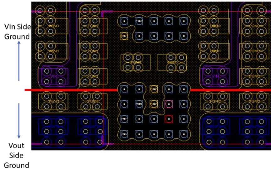
Figure 30. Example of split input-output ground
