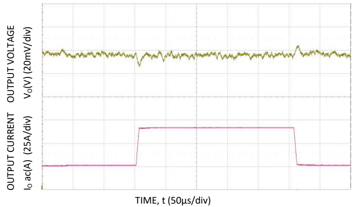
Figure 22. Trans. Resp. to 10A/μs Load Change from 25% to 75% at 12V IN , C_o=4 \times 0.047\mu\text{F} + 4 \times 0.1\mu\text{F} + 15 \times 22\mu\text{F} + 73 \times 47\mu\text{F} + 6 \times 470\mu\text{F} polymer
