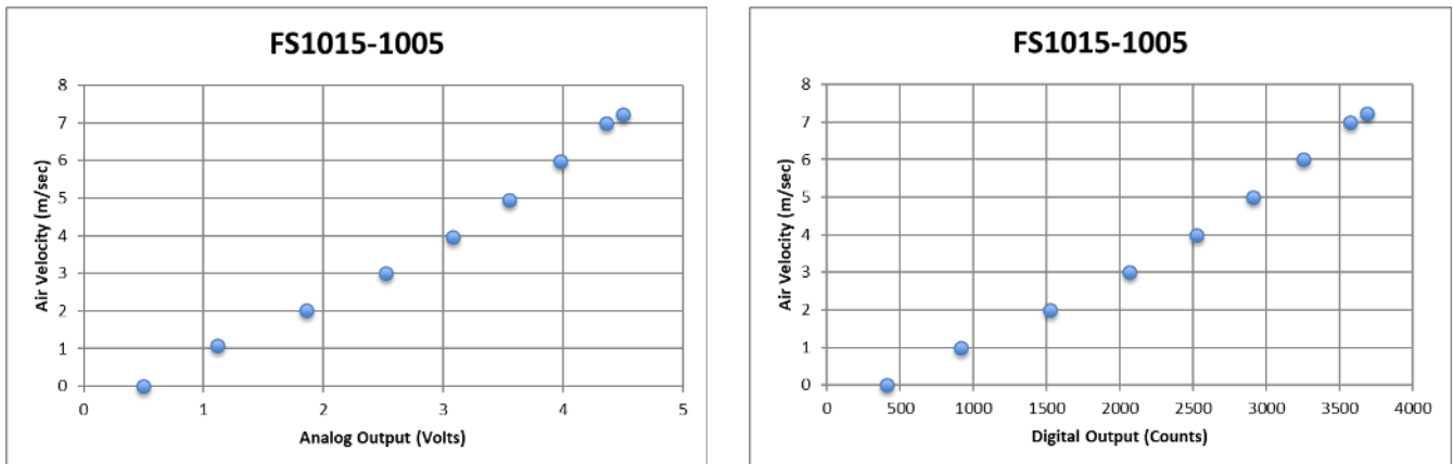
Figure 3. FS1015-1005 Air Velocity Curve
