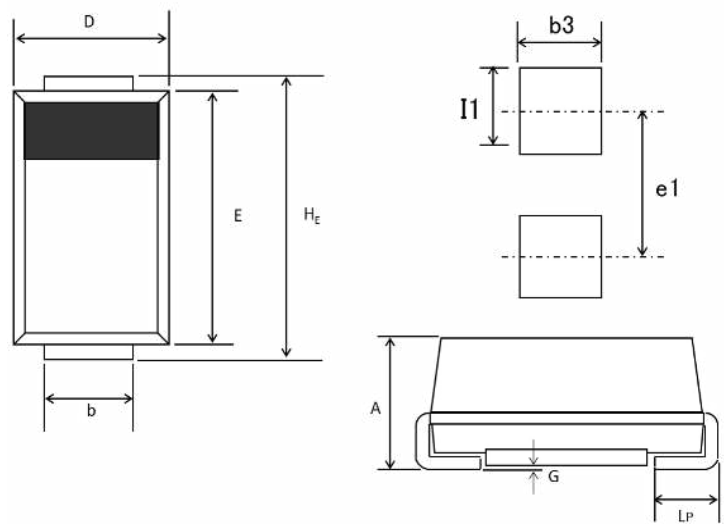
DO-214AC(SMA), (FMDS)
