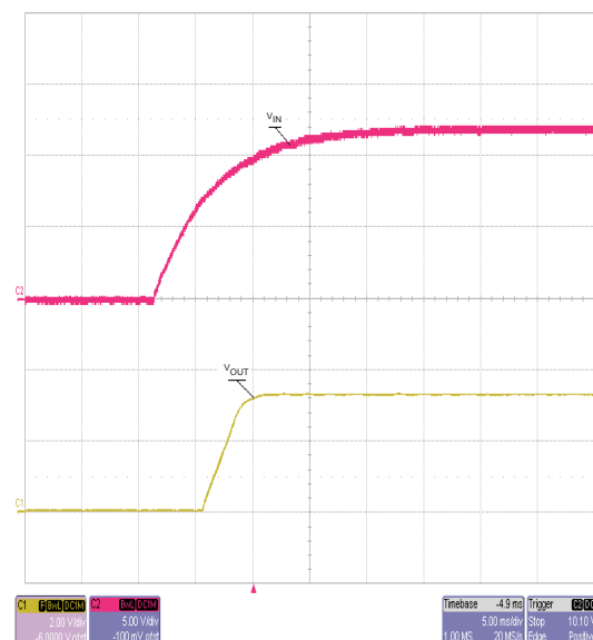
Figure 2-9. TPS54233EVM-373 Start-Up Relative to V_{IN}
