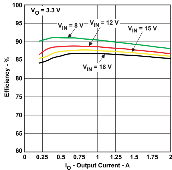
Figure 2-1. TPS54233EVM-373 Efficiency
