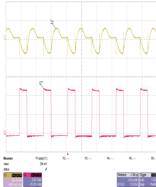
Figure 2-8. TPS54233EVM-373 Input Ripple
