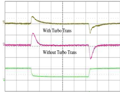
Output voltage response to load current step-change (7.5-22.5-7.5 A) at: T_{ref} = +25^{\circ}C , V_I = 12 V . Top trace: output voltage (100 mV/div.). Middle Trace: output voltage (100mV/div.). Bottom trace: load current (20 A/div.). Time scale: (0.1 ms/div.).
