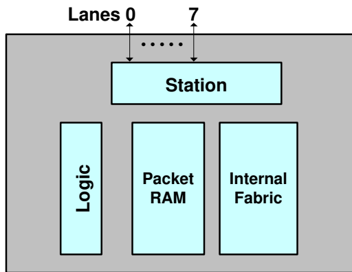
Figure 4-1. PEX 8509 Block Diagram
