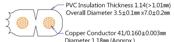
SPT-2 18AWGx2C截面圖 (Wire Cross-Section)
