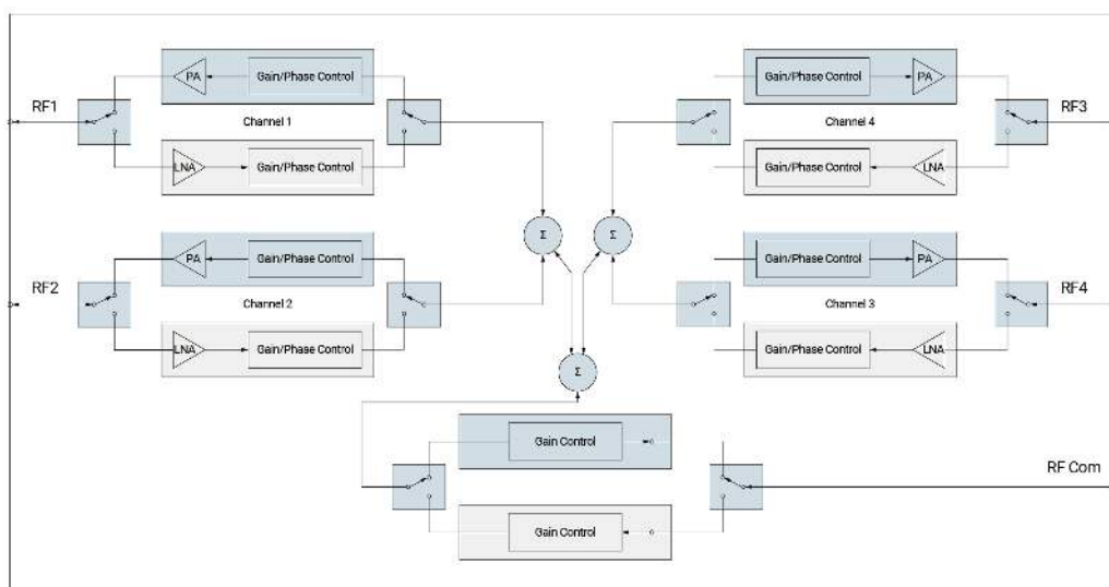
Figure 1. BBoard 5G 39 GHz
