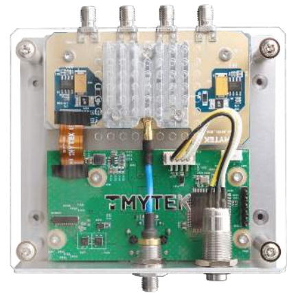
Figure 1. BBoard 5G 39 GHz
