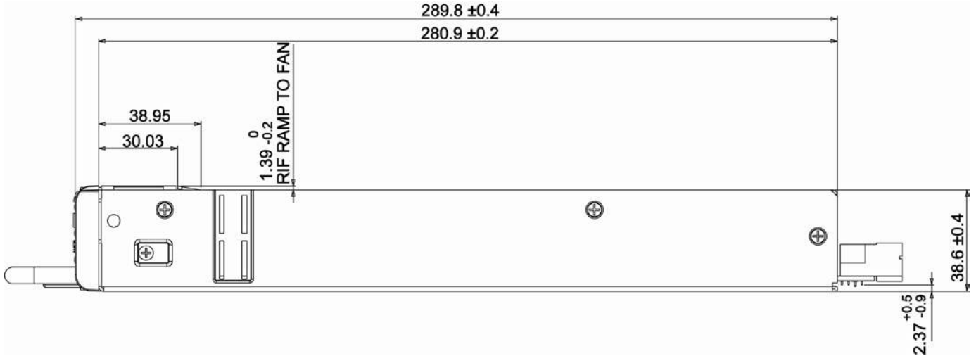
SIDE VIEW
