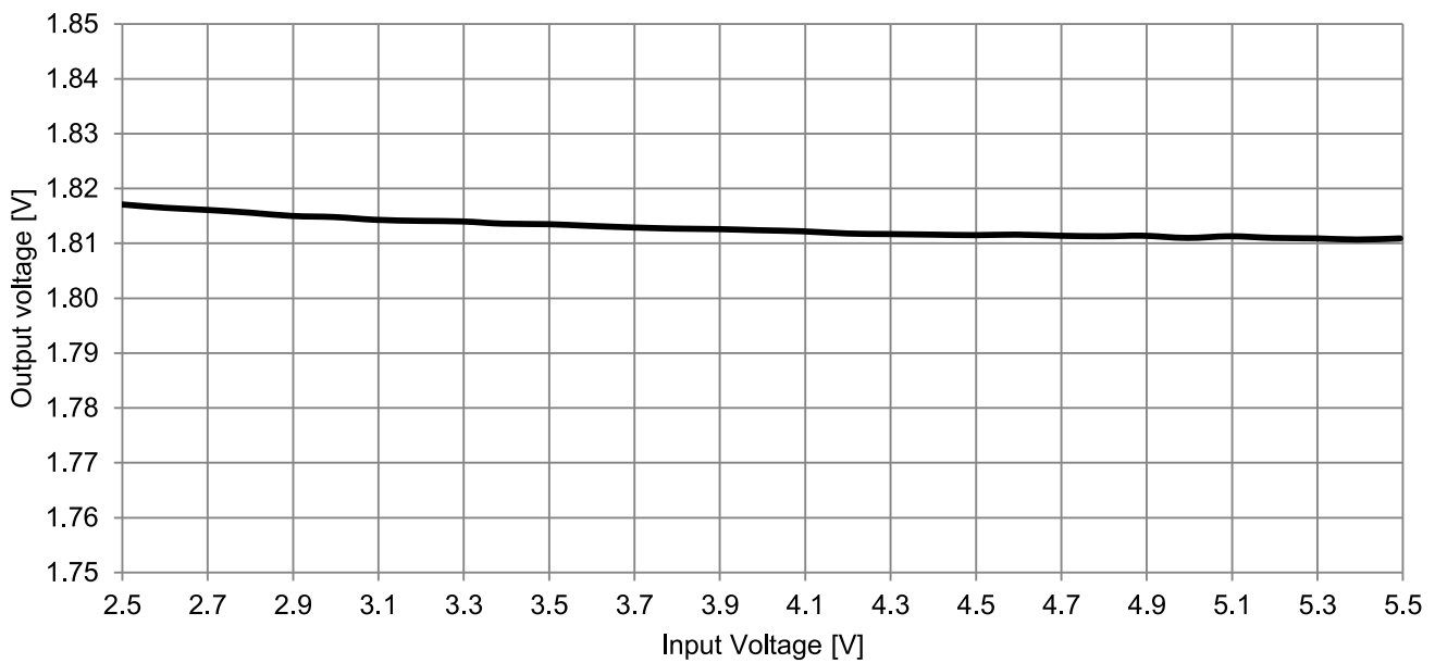
171010501, Line Regulation, V_{OUT} = 1.8V , I_{OUT} = 1A , T_A = 25^\circ C
