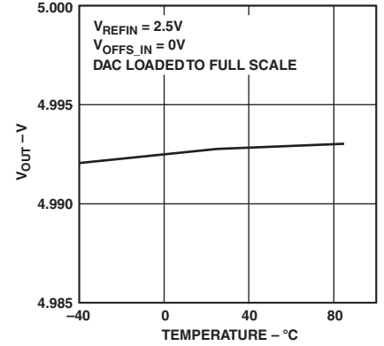
TPC 3. V_{OUT} vs. Temperature
