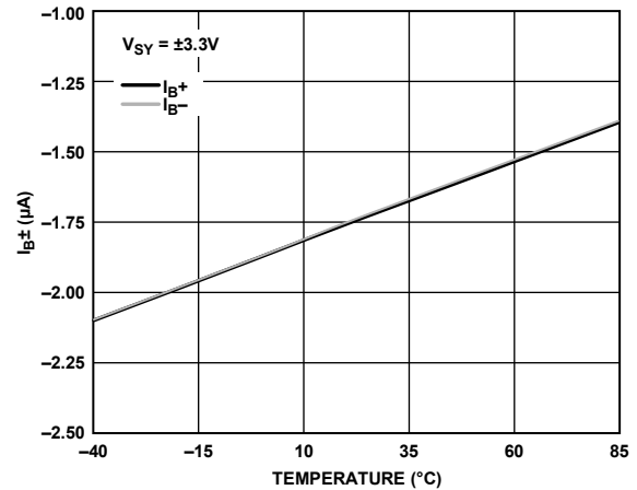
Figure 31. Input Bias Current ( I_{B\pm} ) vs. Temperature, V_{SY} = \pm 3.3\text{ V}
