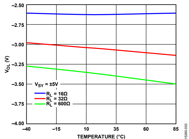
Figure 33. Output Voltage Low ( V_{OL} ) vs. Temperature, V_{SY} = \pm 5\text{ V}
