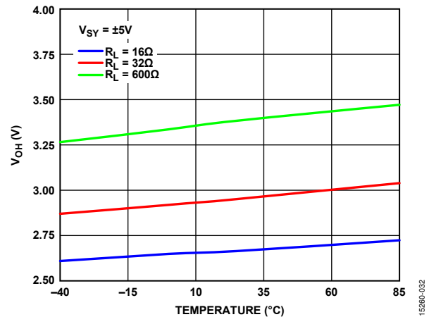
Figure 32. Output Voltage High ( V_{OH} ) vs. Temperature, V_{SY} = \pm 5\text{ V}
