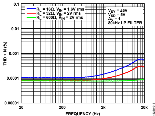
Figure 13. THD + N vs. Frequency, V_{SY} = \pm 5 V
