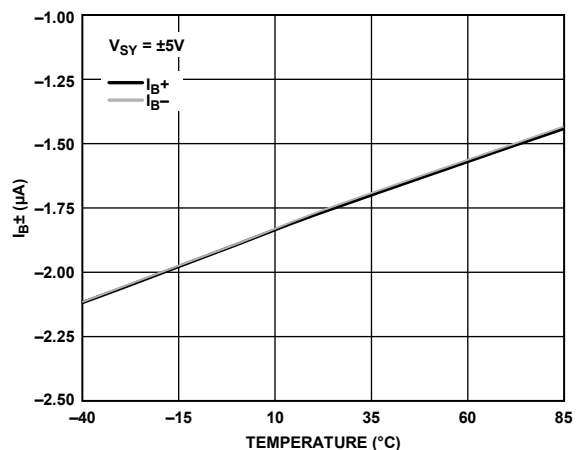
Figure 30. Input Bias Current ( I_{B\pm} ) vs. Temperature, V_{SY} = \pm 5\text{ V}
