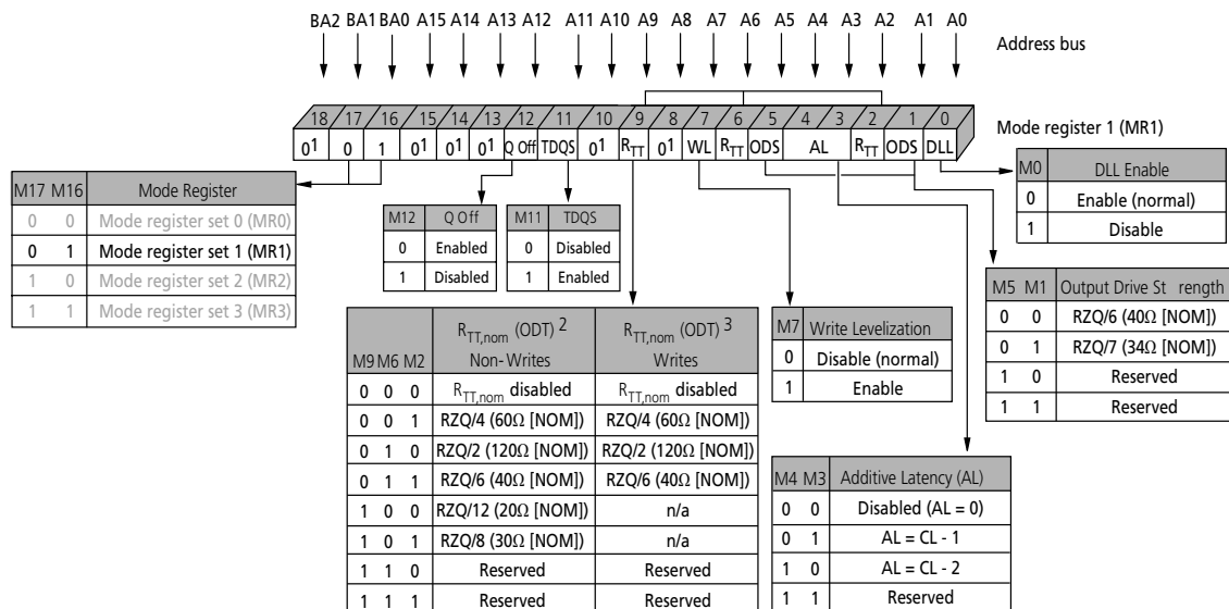
Figure 52: Mode Register 1 (MR1) Definition
