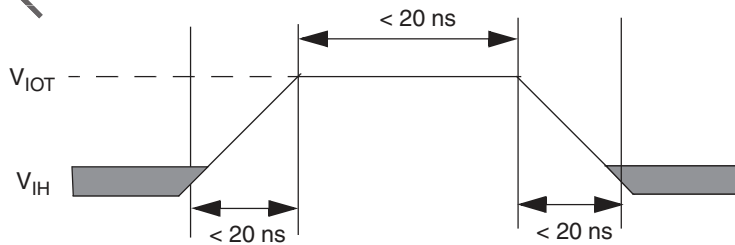
Figure 15. Maximum Positive Overshoot Waveform
