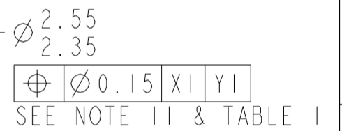
BP HOLE PATTERN COMPONENT SIDE RIGHT POLARIZING GUIDE MODULE BACKPLANE FOOTPRINT
