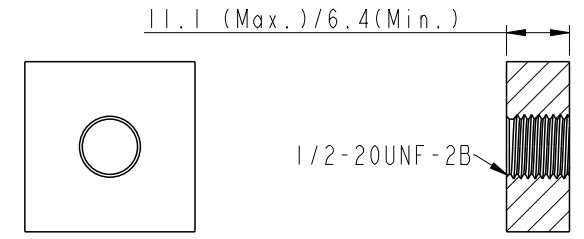
Panel cut out (screw type)
