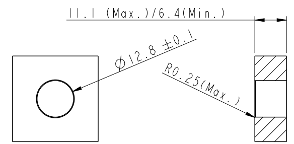
Panel cut out (hole type)
