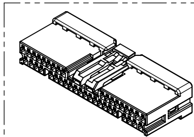
PERSPECTIVE VIEW (REF.)
