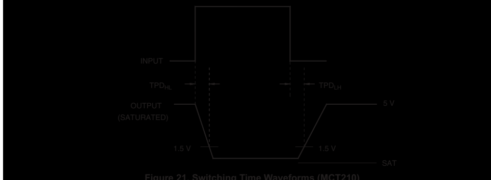
Figure 21. Switching Time Waveforms (MCT210)
